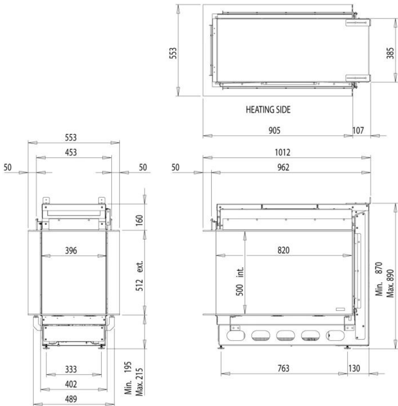
Dimensional Drawing e-MatriX heat 800x500 RD (MkII)
